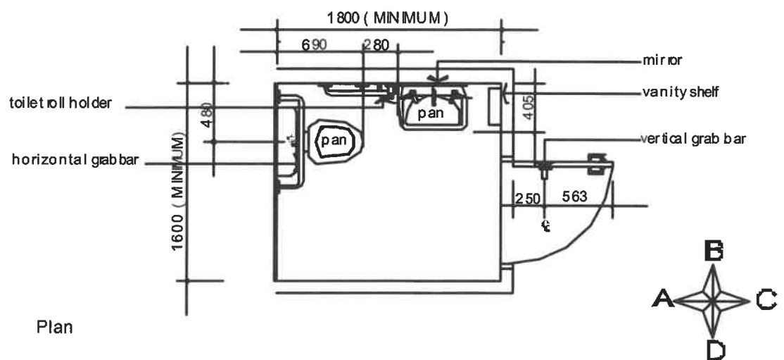
FIGURE 4.1.1 ACCESSIBLE TOILET WITH FLOOR MOUNTED PAN AND CISTERN
